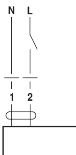
Wiring diagram
